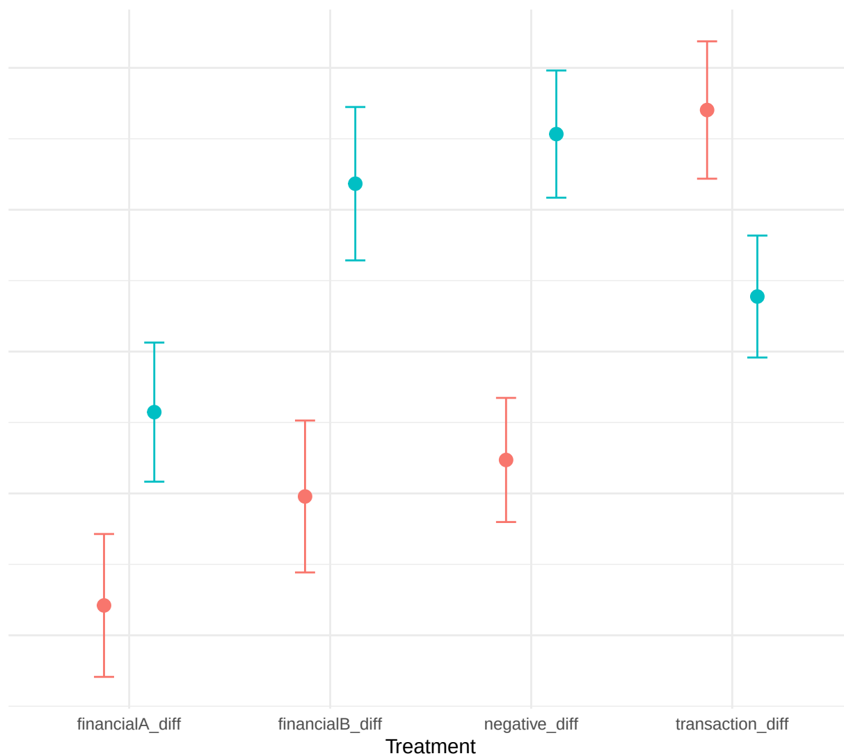
Treatment Effects by Age Group
